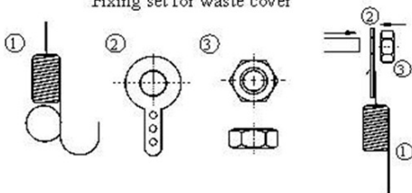
Fixing set for waste cover
