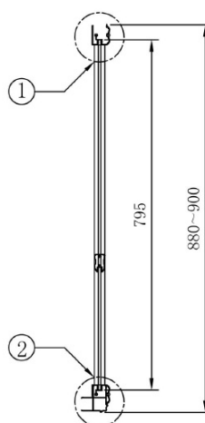
Return Panel 900
