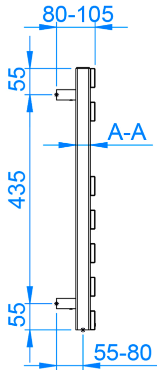
Left View
