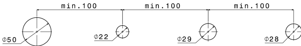
Installation holes
