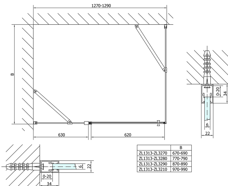
ZL1313L ZL3270L ZL3280L ZL3290L ZL3210L
