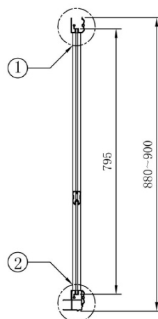
Return Panel 900
