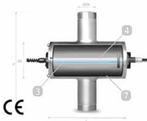
3 - lampa/lamp 4 - křemenné pouzdro/quartz sleeve 7 - komora UV lampy/UV reactor
