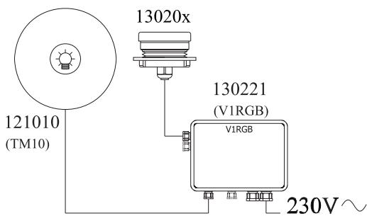
1 13020x chromoterapie s elektronikou 130221 ovládaná tlačítkem TM10. 13020x chromotherapy with control electronics 130221 controlled with TM10 button.
