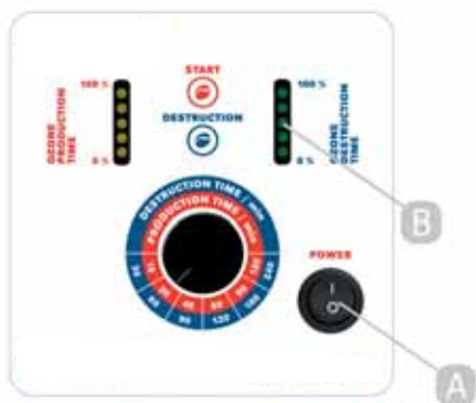
A – Spínač/Switch B – LED indicator/LED Indicator
