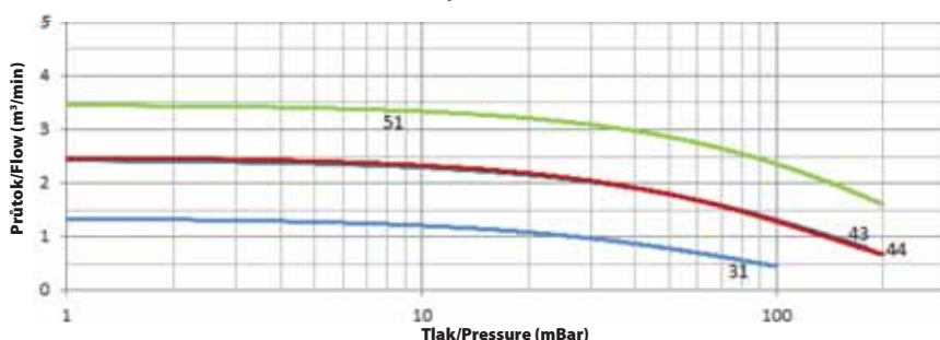
Charakteristika dmychadel/Blowers curve
