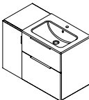
44050 PRACTICO Ceramic Basin 50x40 cm Vanity Base, 2x Drawer 48x54x39 cm CR492-3030 White Glossy CR492-XXXX
